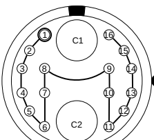
LEMO.FGG.4B.856.ZLA3 KKS16HD Stecker (Lötseite) plug (soldering side)
