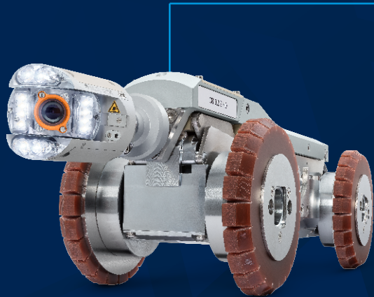
HD Mainline Inspection System ORION ® 3 w/ T76 Camera Tractor
